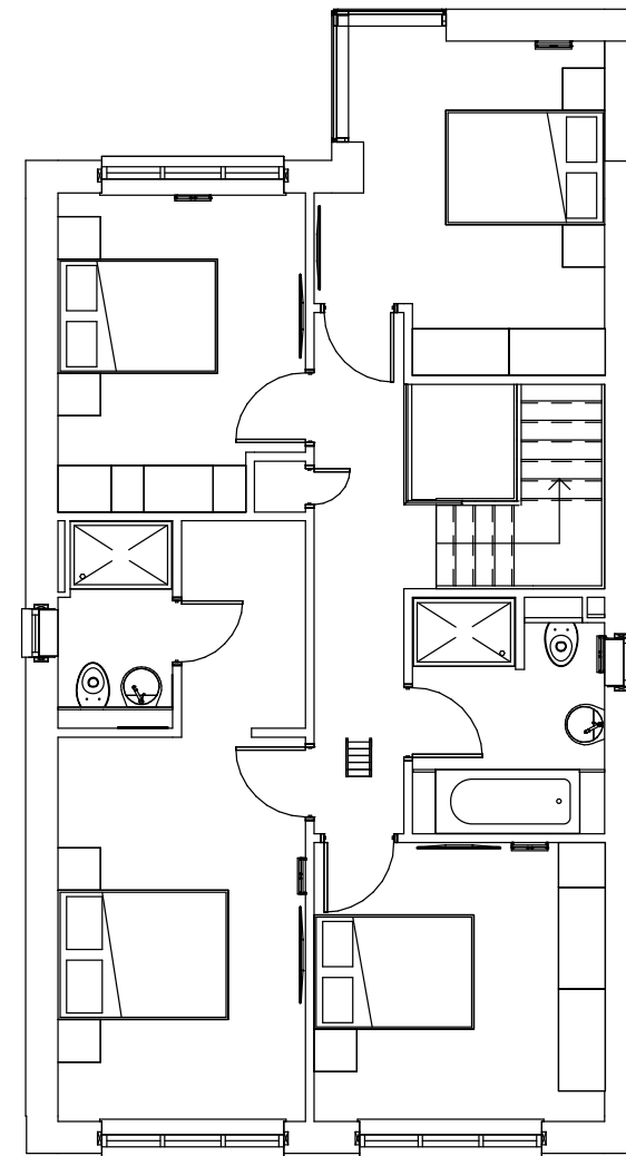
SECOND FLOOR
